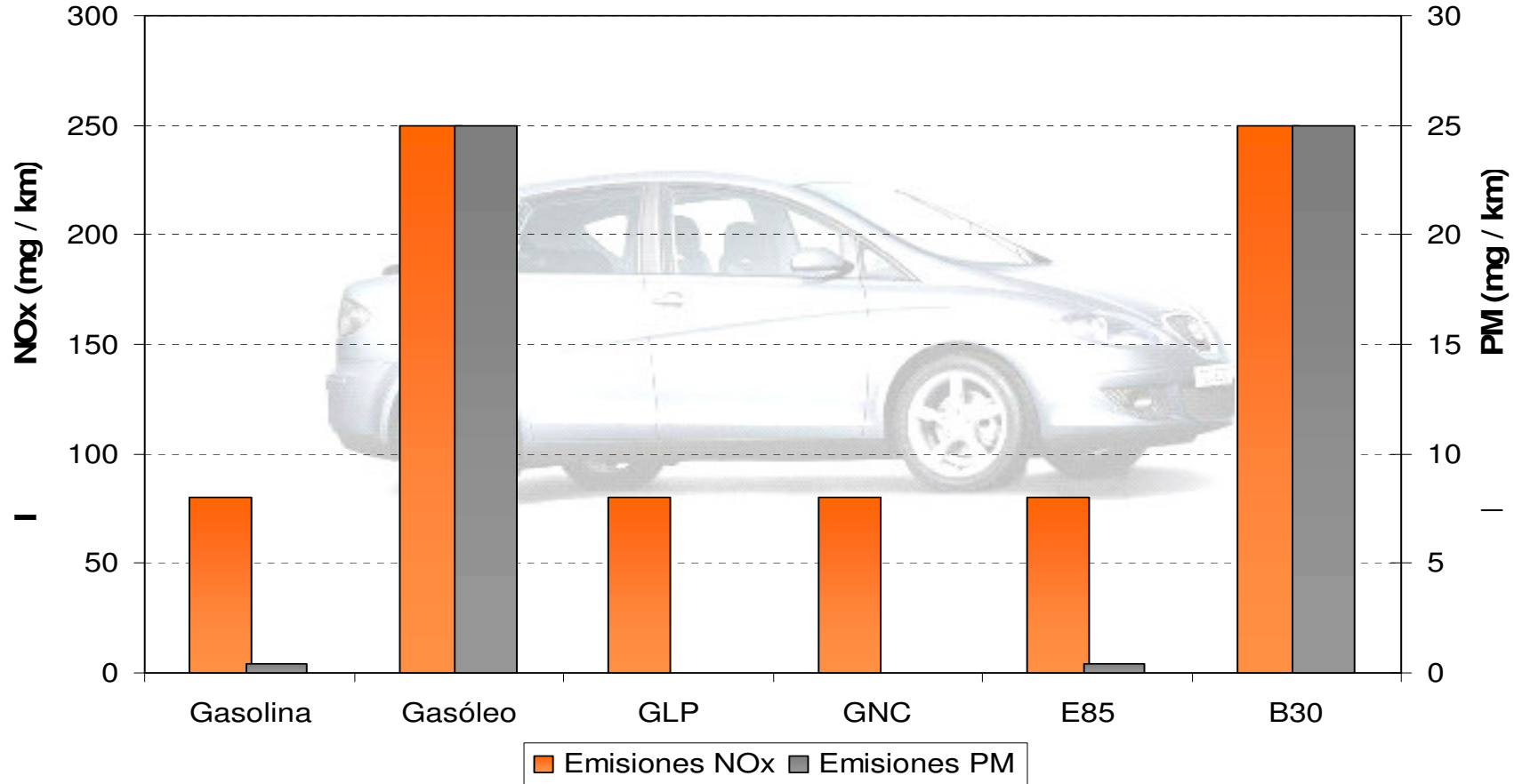
Emissions en escapament Vehicle Euro 4
